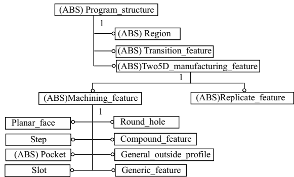
Fig. 11.10 EXPRESS-G diagram for manufacturing features
