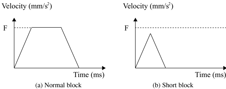
Fig. 4.17 Speed profiles
