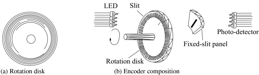
Fig. 1.7 Absolute-type encoder
