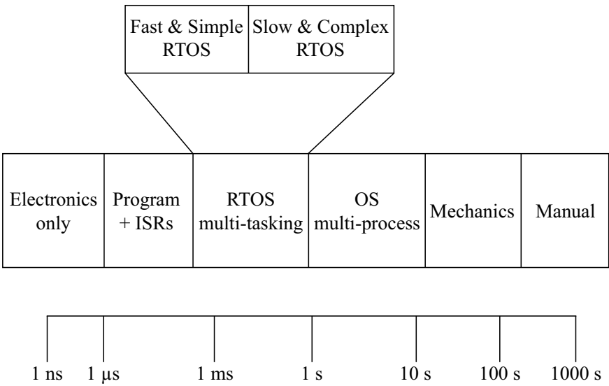
Fig. 9.1 Time spectrum of a real-time system
