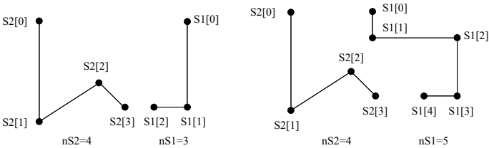
Fig. 8.26 Divided profiles
