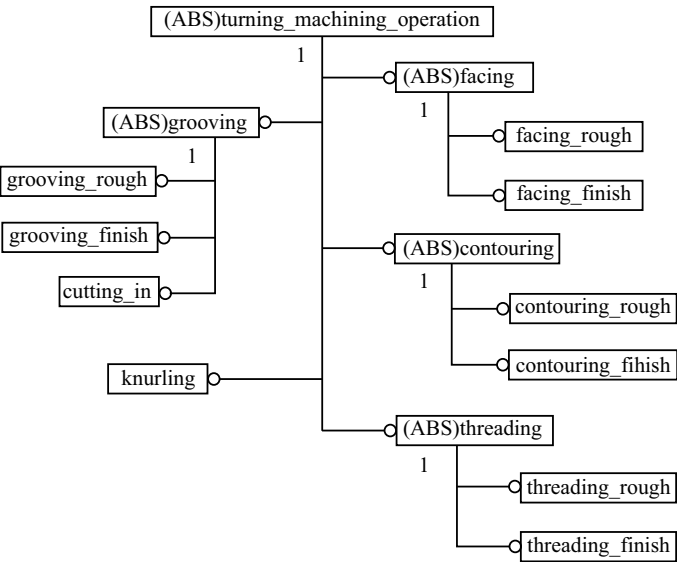
Fig. 11.14 EXPRESS-G diagram for turning_machining_operation
