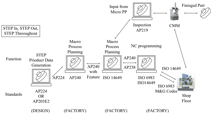
Fig. 11.4 Suite of STEP-Manufacturing
