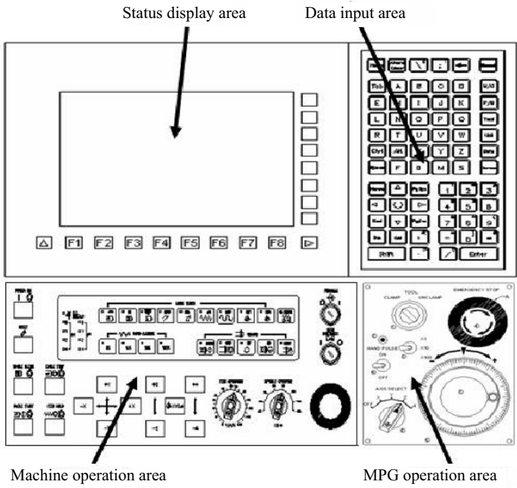
Fig. 8.1 Typical operation panel
