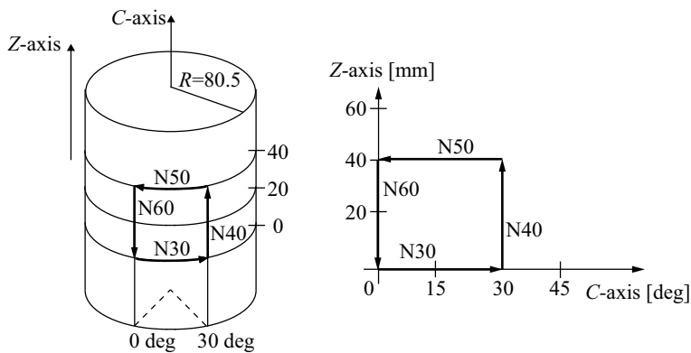
Fig. 2.12 Cylindrical interpolation
