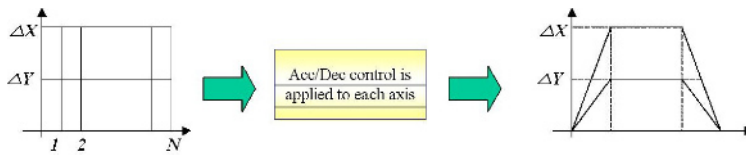
Fig. 4.2 Change to pulse profile after Acc/Dec control
