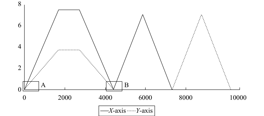
Fig. 6.16 Fine interpolation
