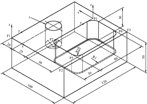
Fig. 11.17 Simple example test part for milling
