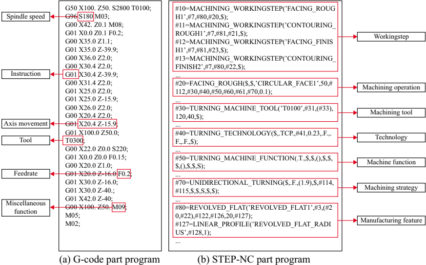
Fig. 11.2 Comparison of G-code part program and STEP-NC part program
