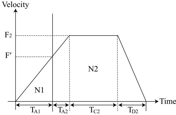
Fig. 4.22 Speed profiles for short block/normal block with identical feedrates
